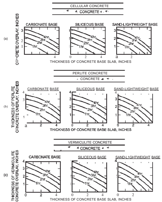
FIGURE 721.2.2.3(1) FIRE-RESISTANCE RATINGS FOR CONCRETE ROOF ASSEMBLIES
