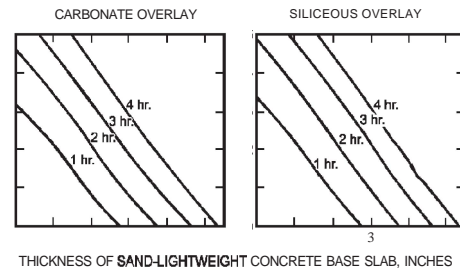
FIGURE 721.2.2.2 FIRE-RESISTANCE RATINGS FOR TWO-COURSE CONCRETE FLOORS
