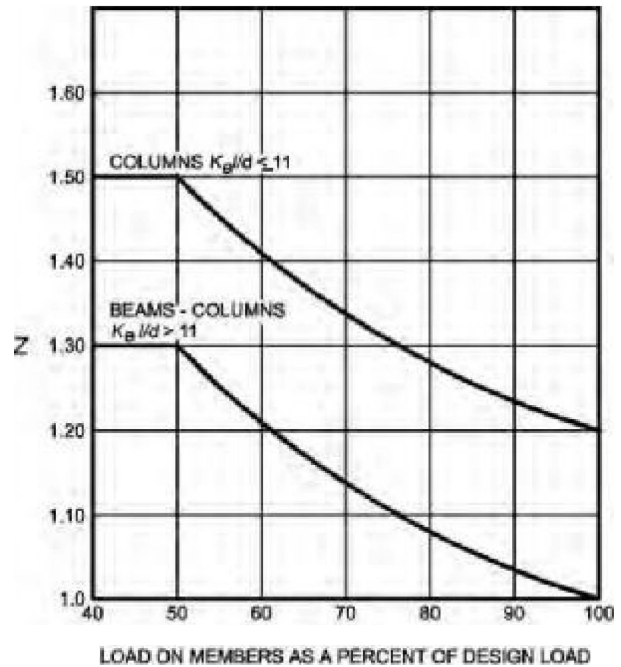
FIGURE 721.6.3(1) LOAD FIGURE
