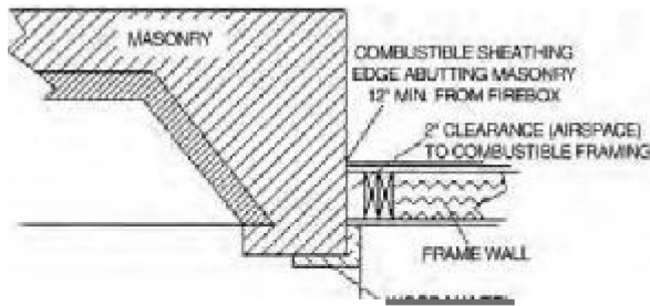
FIGURE 2111.11 ILLUSTRATION OF EXCEPTION TO FIREPLACE CLEARANCE PROVISION
