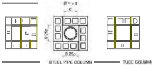
FIGURE 721.5.1(7) CONCRETE OR CLAY MASONRY PROTECTED STRUCTURAL STEEL COLUMNS
