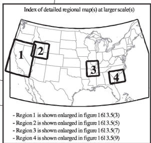
FIGURE 1613.5(1) MAXIMUM CONSIDERED EARTHQUAKE GROUND MOTION FOR THE CONTERMINOUS UNITED STATES OF 0.2 SEC SPECTRAL RESPONSE ACCELERATION (5% OF CRITICAL DAMPING), SITE CLASS B
