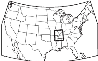
FIGURE 1613.5(8) MAXIMUM CONSIDERED EARTHQUAKE GROUND MOTION FOR REGION 3 OF 1.0 SEC SPECTRAL RESPONSE ACCELERATION (5% OF CRITICAL DAMPING), SITE CLASS B
