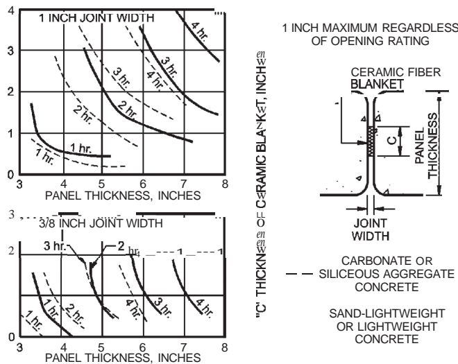
FIGURE 721.2.1.3.1 CERAMIC FIBER JOINT PROTECTION
