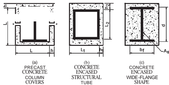
FIGURE 721.5.1(6) CONCRETE PROTECTED STRUCTURAL STEEL COLUMNSa,b
