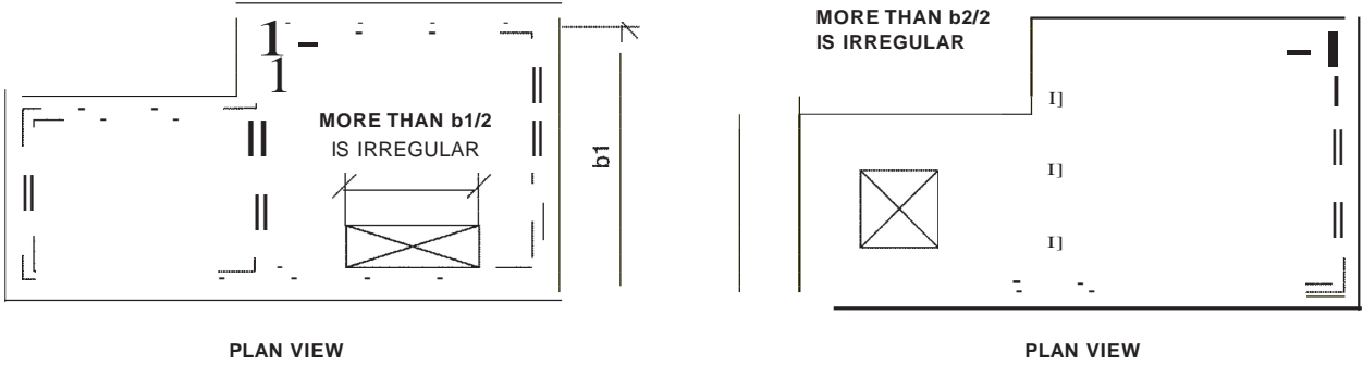
FIGURE 2308.12.6(8) OPENING LIMITATIONS FOR FLOOR AND ROOF DIAPHRAGMS
