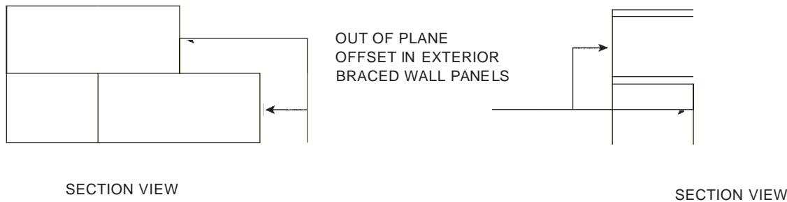
FIGURE 2308.12.6(1) BRACED WALL PANELS OUT OF PLANE
