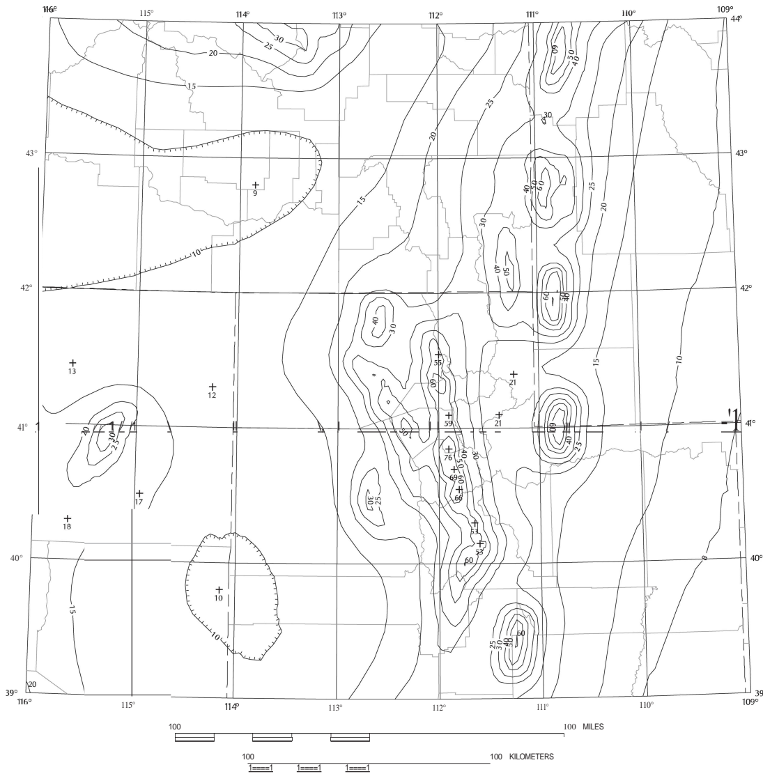
FIGURE 1613.5(6) MAXIMUM CONSIDERED EARTHQUAKE GROUND MOTION FOR REGION 2 OF 1.0 SEC SPECTRAL RESPONSE ACCELERATION (5% OF CRITICAL DAMPING), SITE CLASS B
