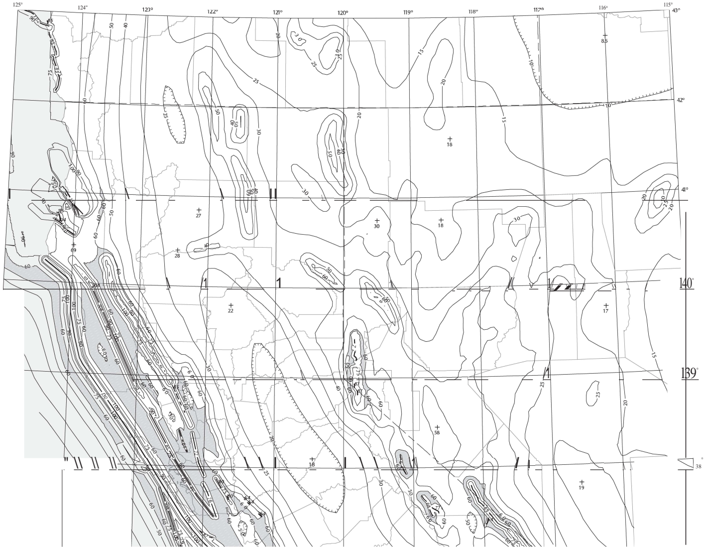
FIGURE 1613.5(4) MAXIMUM CONSIDERED EARTHQUAKE GROUND MOTION FOR REGION 1 OF 1.0 SEC SPECTRAL RESPONSE ACCELERATION (5% OF CRITICAL DAMPING), SITE CLASS B
